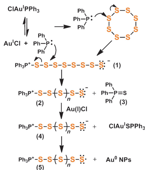
Scheme 2. Proposed mechanism for the formation of AuNPs in liquid sulfur using \text{ClAu}^{\text{I}}\text{PPh}_3 .
