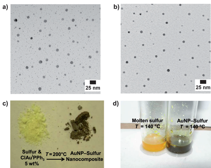
Figure 2. a) Transmission electron micrograph of AuNPs with diameters of 5.1 \pm 3 nm formed directly in liquid sulfur using 5 wt % ClAu I PPh 3 . b) Transmission electron micrograph of AuNPs with diameters of 6.9 \pm 2 nm formed using 50 wt % ClAu I PPh 3 by predissolution with sulfur using CS 2 and removal of the solvent. c) Digital image of the sulfur–ClAu I PPh 3 reaction mixture before (left) and after AuNP formation (right) at 200 °C and cooled to room temperature. d) Neat liquid sulfur at 140 °C below floor temperature for the ring-opening polymerization (left) and the molten form of AuNP–sulfur nanocomposites formed at 200 °C, cooled to room temperature, and re-melted at 140 °C (right).
